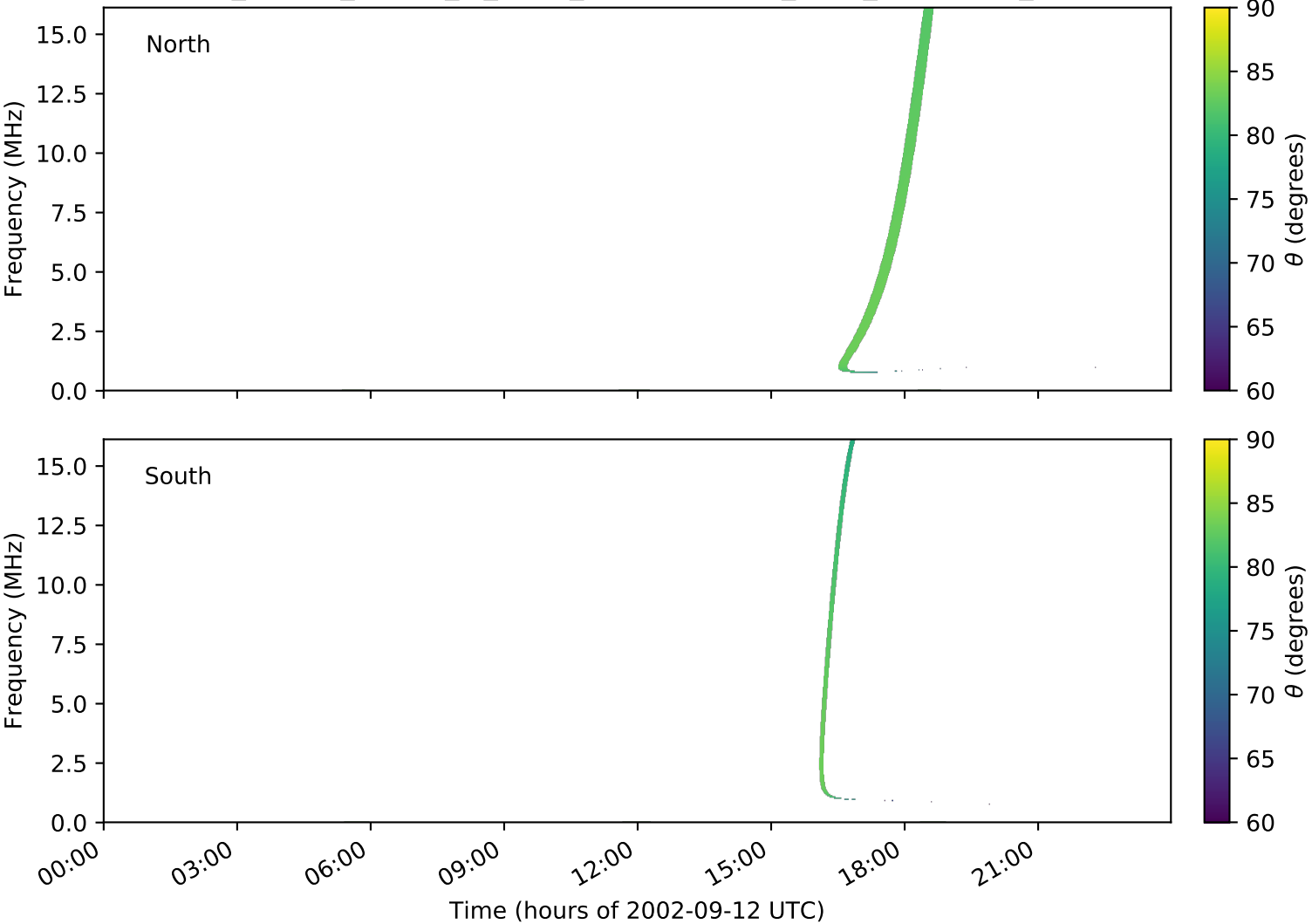
expres_cassini_jupiter_io_isaac_lossc-wid1deg_3kev_20020912_v01.cdf
