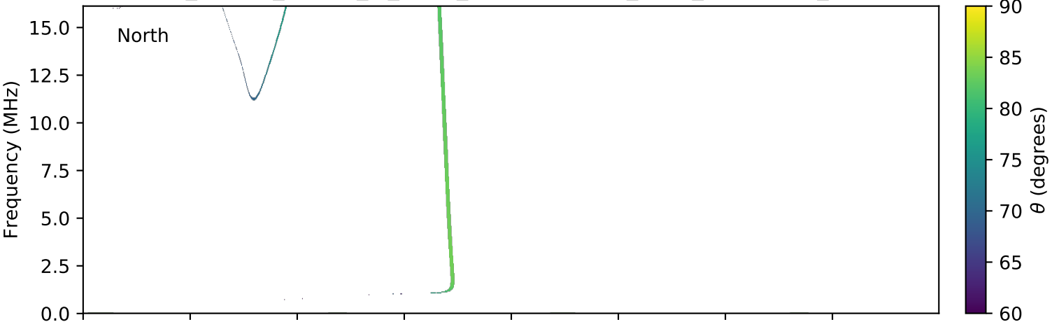
expres_cassini_jupiter_io_isaac_lossc-wid1deg_3kev_20020906_v01.cdf
