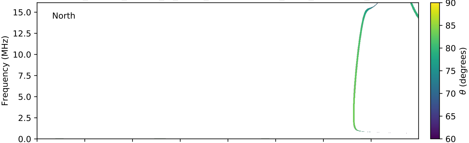
expres_cassini_jupiter_io_isaac_lossc-wid1deg_3kev_20020903_v01.cdf
