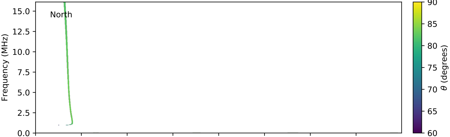
expres_cassini_jupiter_io_isaac_lossc-wid1deg_3kev_20020901_v01.cdf
