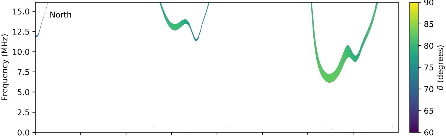
expres_cassini_jupiter_ganymede_isaac_lossc-wid1deg_3kev_20020926_v01.cdf
