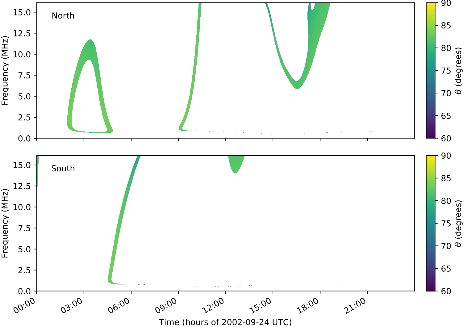
expres_cassini_jupiter_ganymede_isaac_lossc-wid1deg_3kev_20020924_v01.cdf
