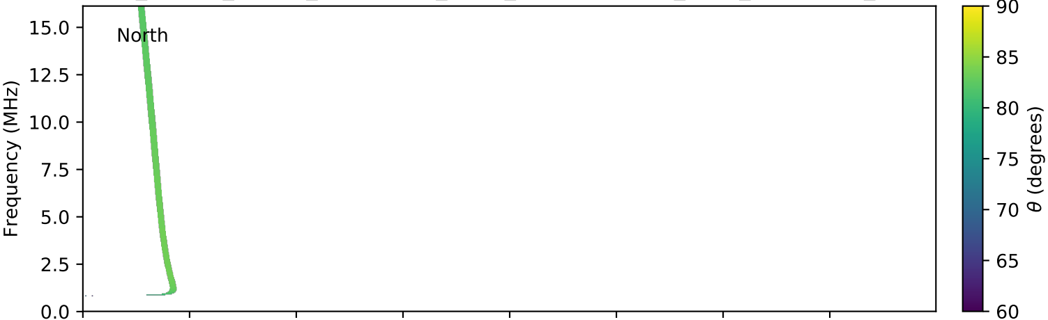
expres_cassini_jupiter_ganymede_isaac_lossc-wid1deg_3kev_20020920_v01.cdf
