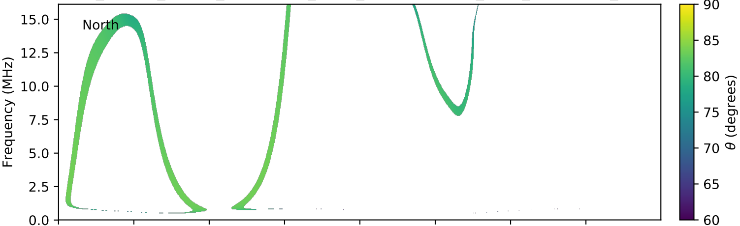
expres_cassini_jupiter_ganymede_isaac_lossc-wid1deg_3kev_20020917_v01.cdf
