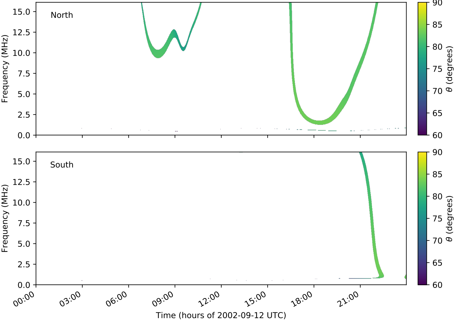
expres_cassini_jupiter_ganymede_isaac_lossc-wid1deg_3kev_20020912_v01.cdf
