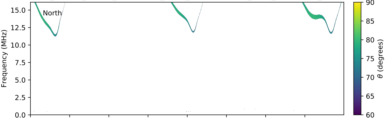
expres_cassini_jupiter_ganymede_isaac_lossc-wid1deg_3kev_20020911_v01.cdf
