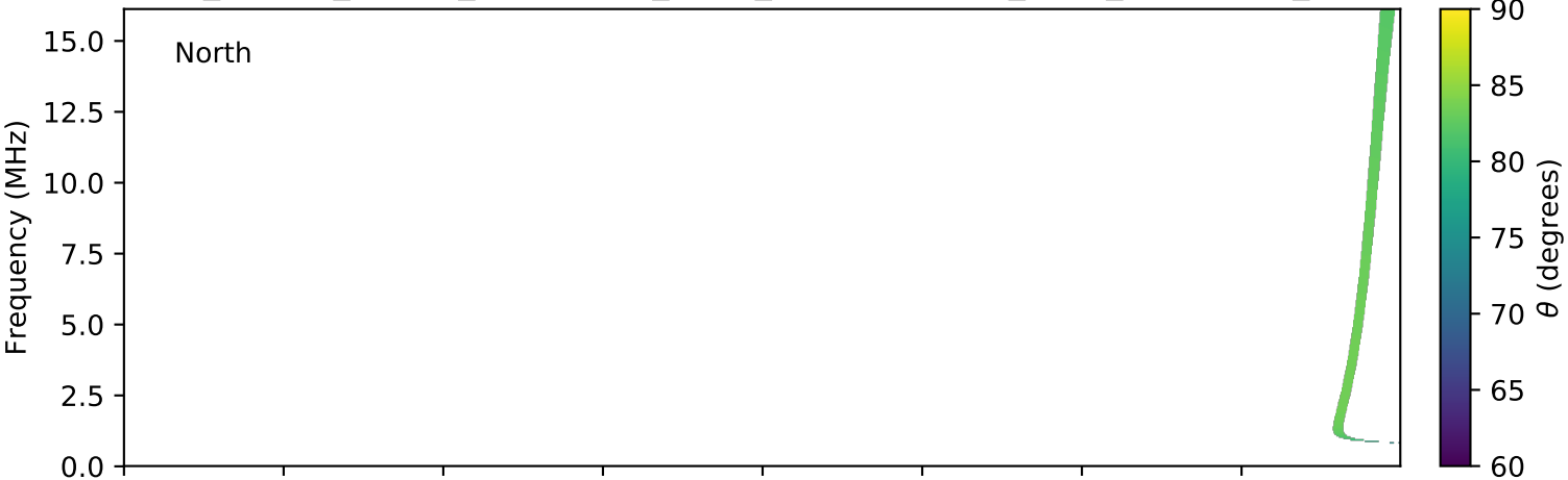
expres_cassini_jupiter_ganymede_isaac_lossc-wid1deg_3kev_20020909_v01.cdf
