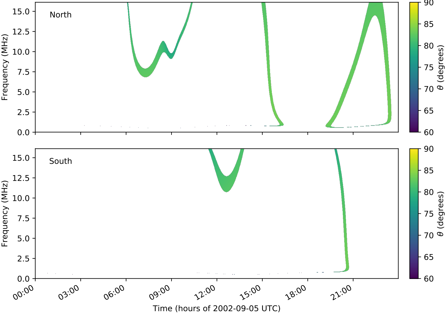
expres_cassini_jupiter_ganymede_isaac_lossc-wid1deg_3kev_20020905_v01.cdf
