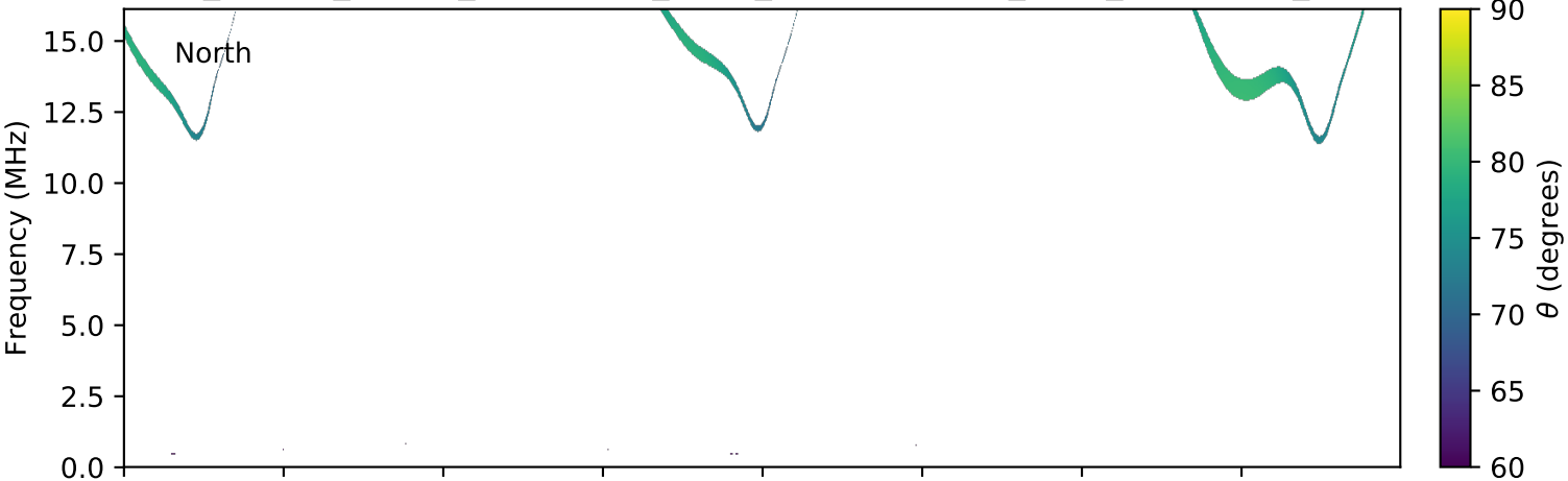
expres_cassini_jupiter_ganymede_isaac_lossc-wid1deg_3kev_20020904_v01.cdf
