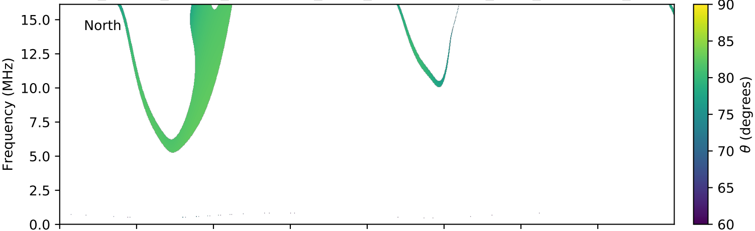
expres_cassini_jupiter_ganymede_isaac_lossc-wid1deg_3kev_20020903_v01.cdf
