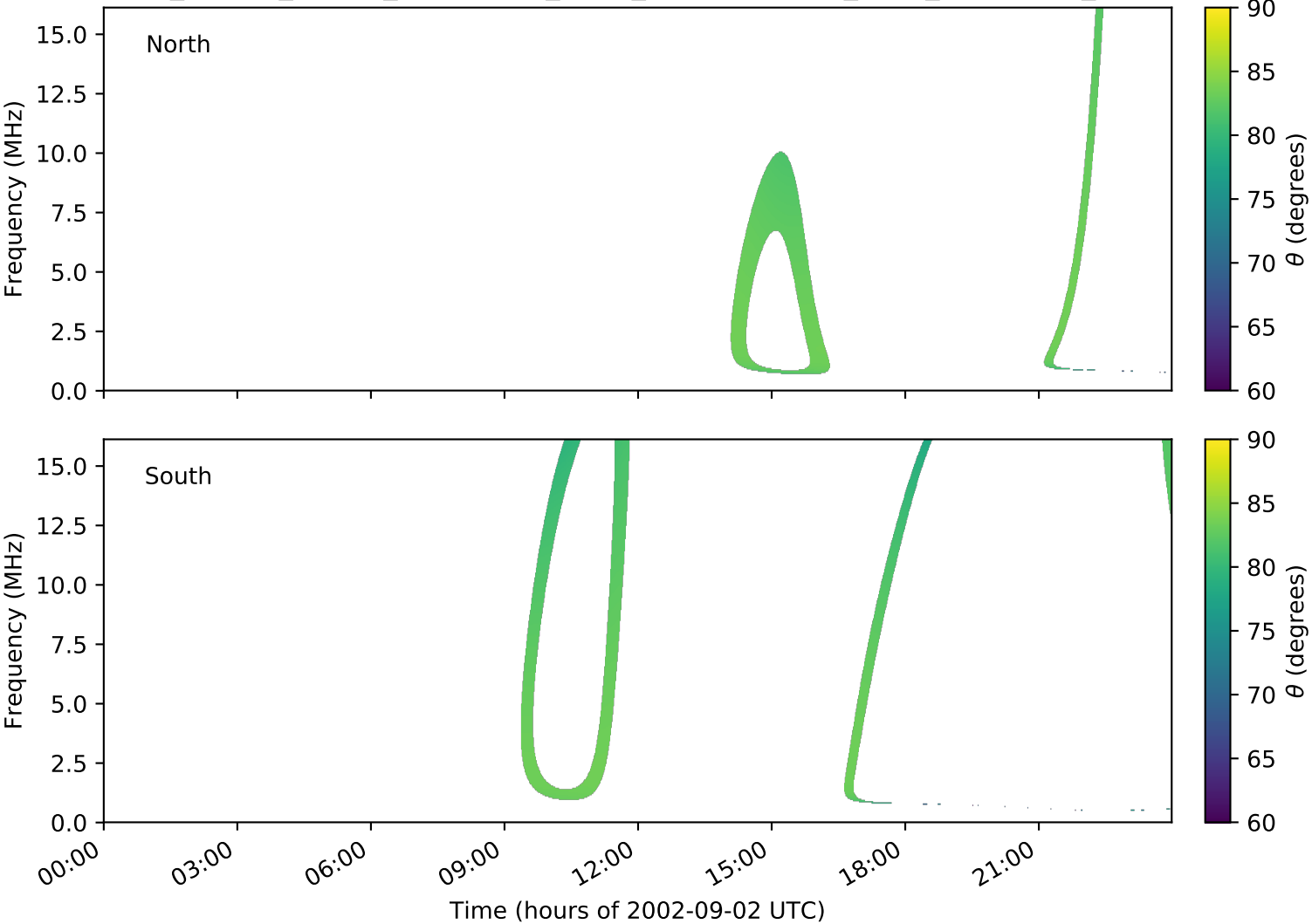
expres_cassini_jupiter_ganymede_isaac_lossc-wid1deg_3kev_20020902_v01.cdf
