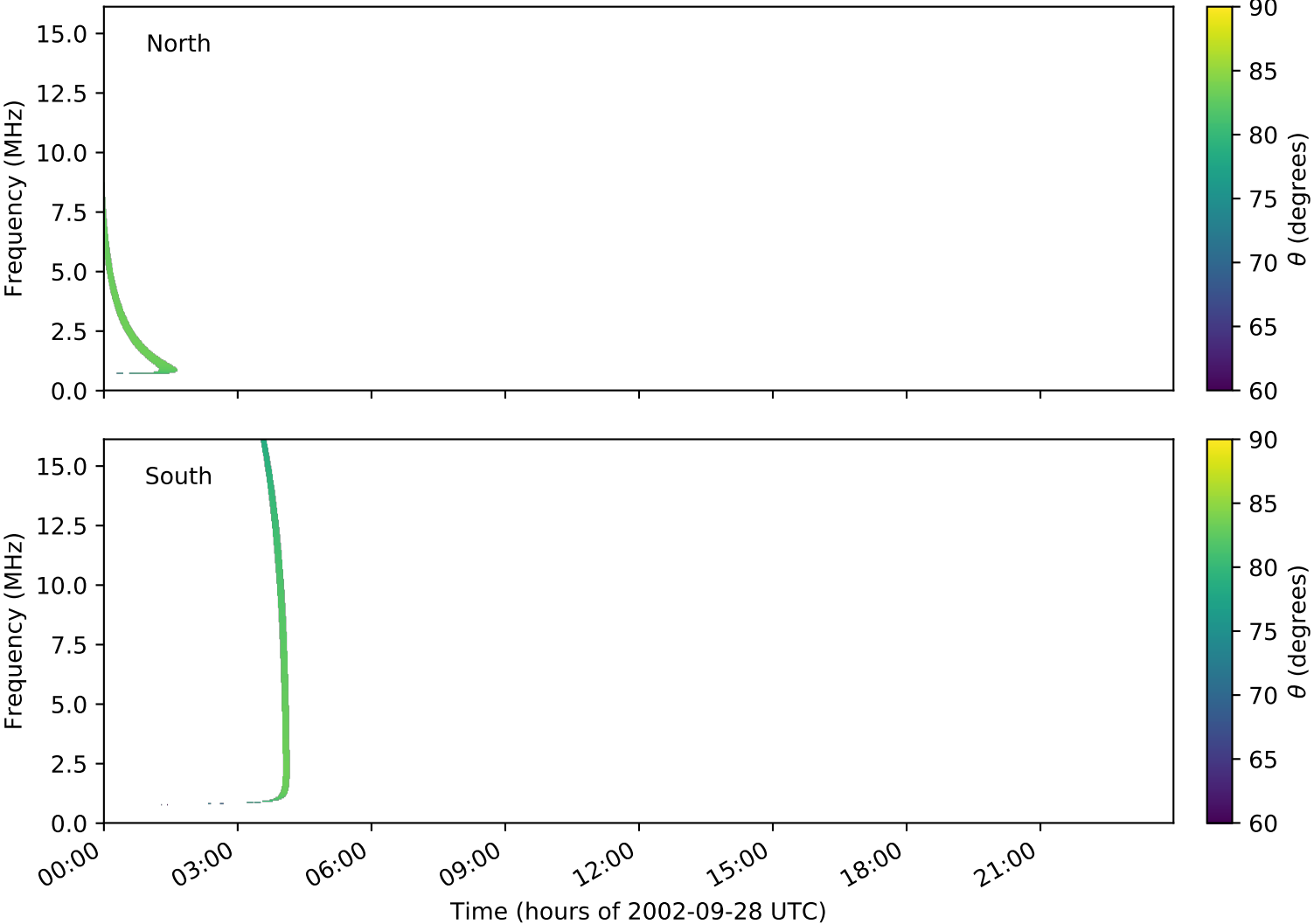
expres_cassini_jupiter_europa_isaac_lossc-wid1deg_3kev_20020928_v01.cdf
