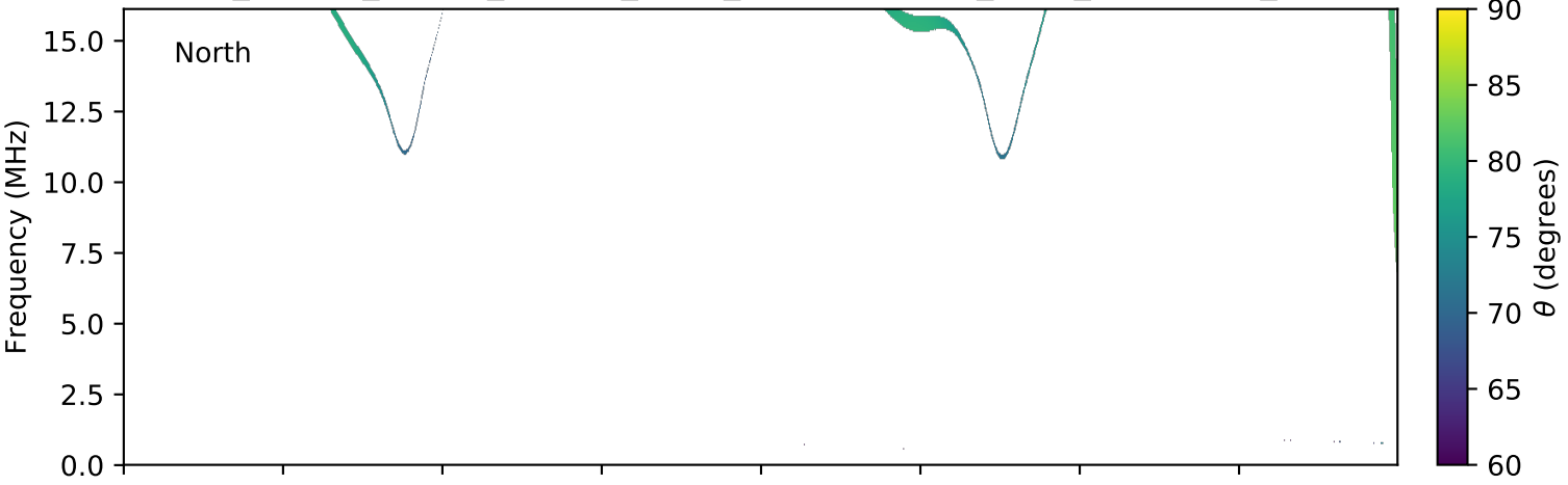
expres_cassini_jupiter_europa_isaac_lossc-wid1deg_3kev_20020927_v01.cdf
