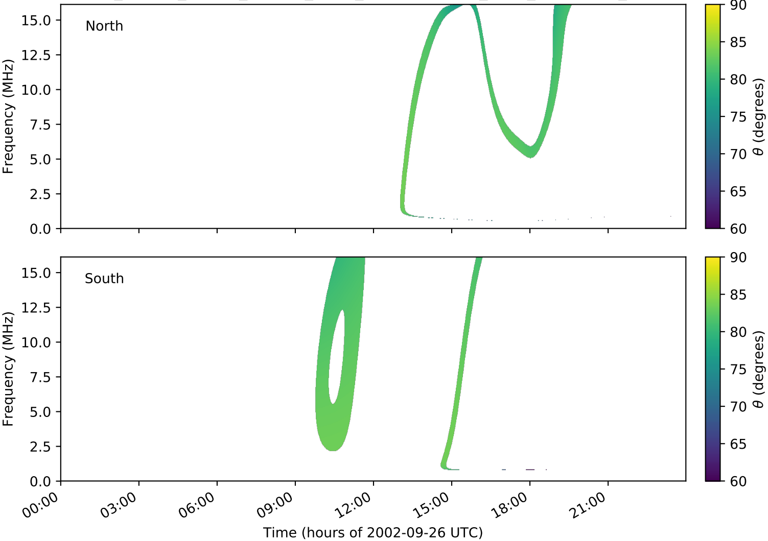
expres_cassini_jupiter_europa_isaac_lossc-wid1deg_3kev_20020926_v01.cdf
