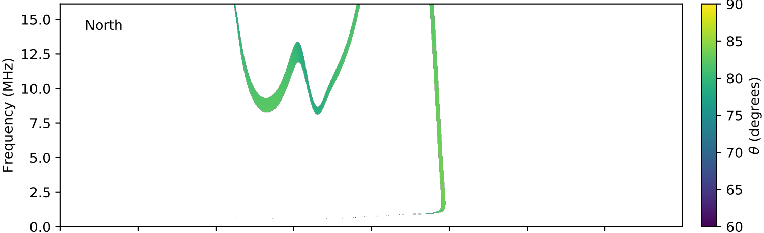
expres_cassini_jupiter_europa_isaac_lossc-wid1deg_3kev_20020924_v01.cdf
