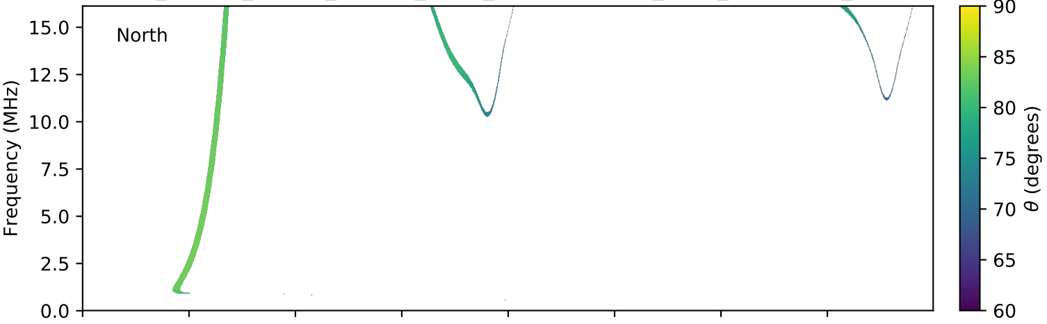
expres_cassini_jupiter_europa_isaac_lossc-wid1deg_3kev_20020923_v01.cdf
