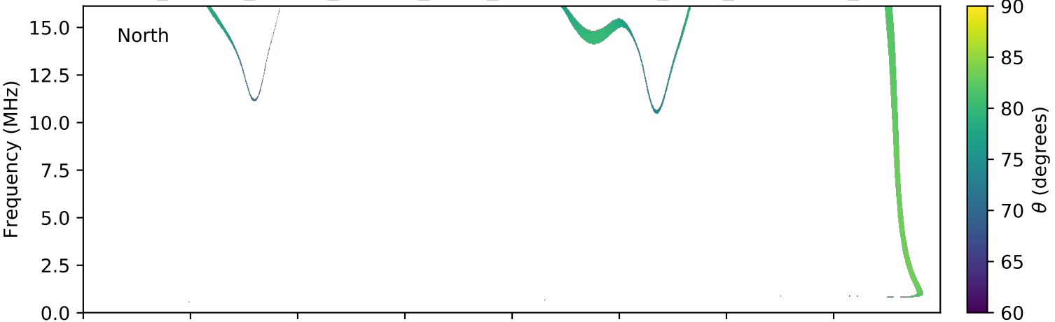
expres_cassini_jupiter_europa_isaac_lossc-wid1deg_3kev_20020920_v01.cdf
