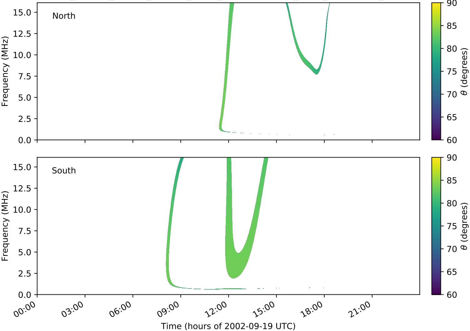
expres_cassini_jupiter_europa_isaac_lossc-wid1deg_3kev_20020919_v01.cdf
