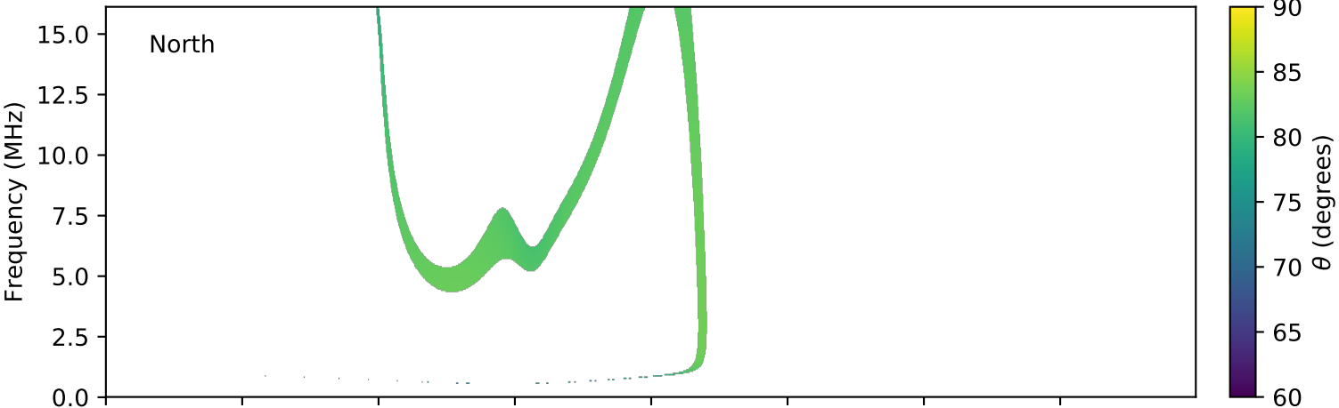
expres_cassini_jupiter_europa_isaac_lossc-wid1deg_3kev_20020917_v01.cdf
