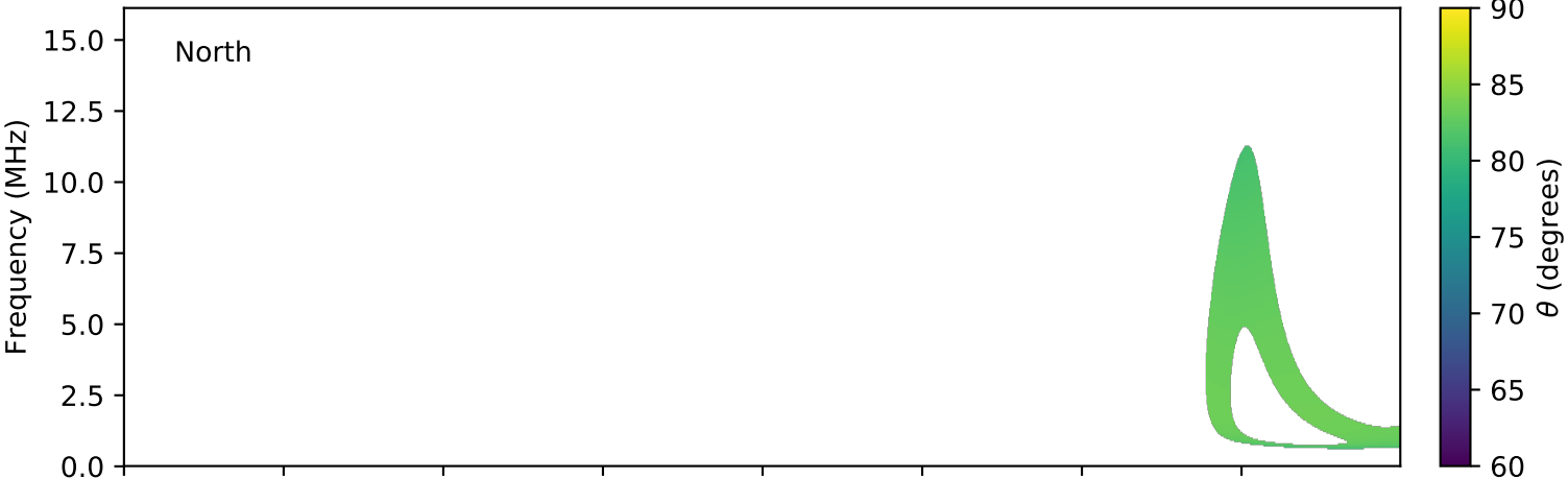
expres_cassini_jupiter_europa_isaac_lossc-wid1deg_3kev_20020915_v01.cdf
