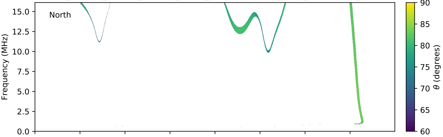
expres_cassini_jupiter_europa_isaac_lossc-wid1deg_3kev_20020913_v01.cdf
