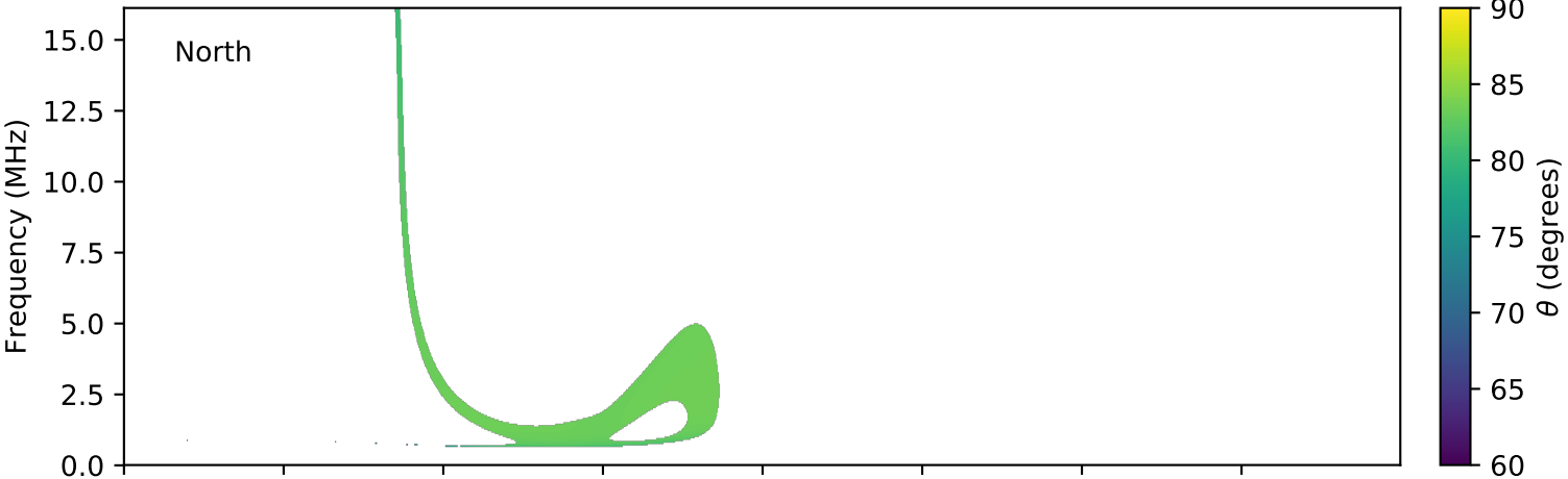
expres_cassini_jupiter_europa_isaac_lossc-wid1deg_3kev_20020910_v01.cdf
