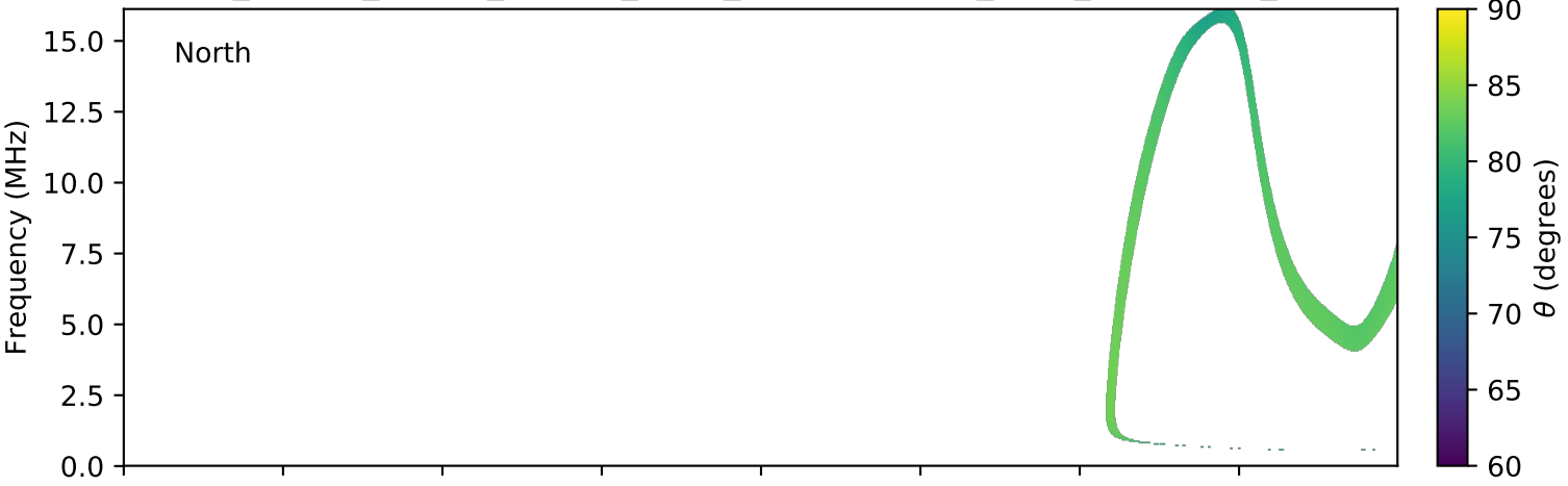
expres_cassini_jupiter_europa_isaac_lossc-wid1deg_3kev_20020908_v01.cdf
