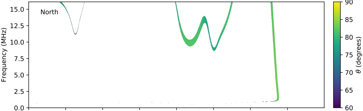
expres_cassini_jupiter_europa_isaac_lossc-wid1deg_3kev_20020906_v01.cdf
