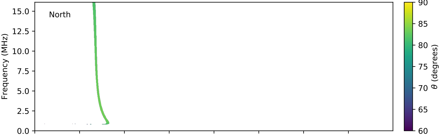
expres_cassini_jupiter_europa_isaac_lossc-wid1deg_3kev_20020903_v01.cdf
