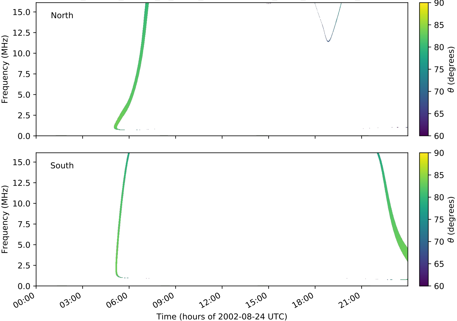
expres_cassini_jupiter_io_isaac_lossc-wid1deg_3kev_20020824_v01.cdf
