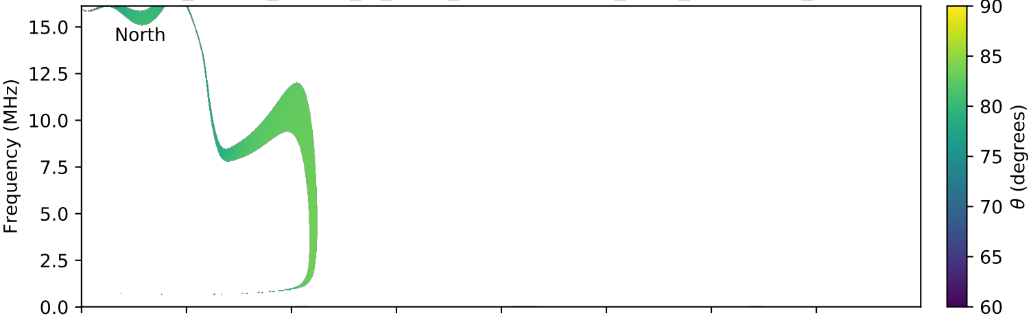
expres_cassini_jupiter_io_isaac_lossc-wid1deg_3kev_20020823_v01.cdf
