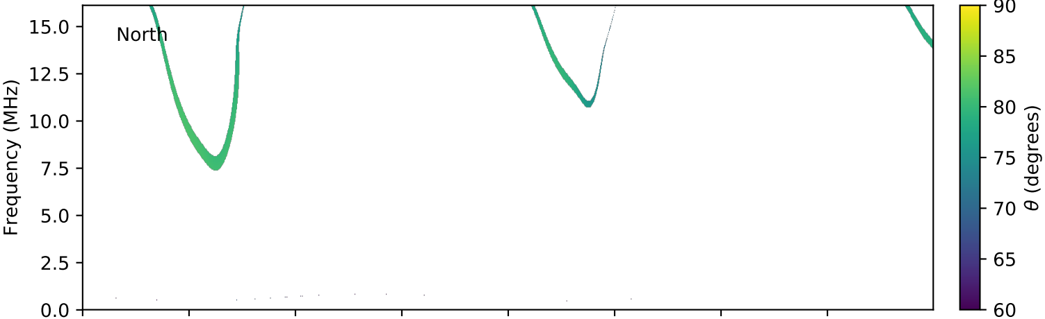
expres_cassini_jupiter_ganymede_isaac_lossc-wid1deg_3kev_20020827_v01.cdf
