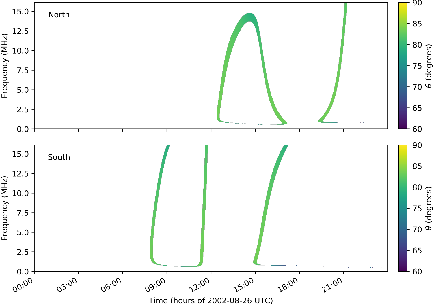
expres_cassini_jupiter_ganymede_isaac_lossc-wid1deg_3kev_20020826_v01.cdf
