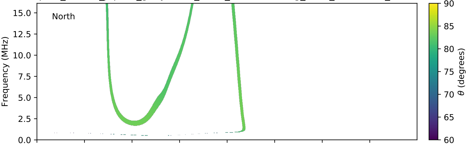
expres_cassini_jupiter_ganymede_isaac_lossc-wid1deg_3kev_20020822_v01.cdf
