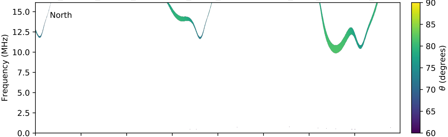
expres_cassini_jupiter_ganymede_isaac_lossc-wid1deg_3kev_20020821_v01.cdf
