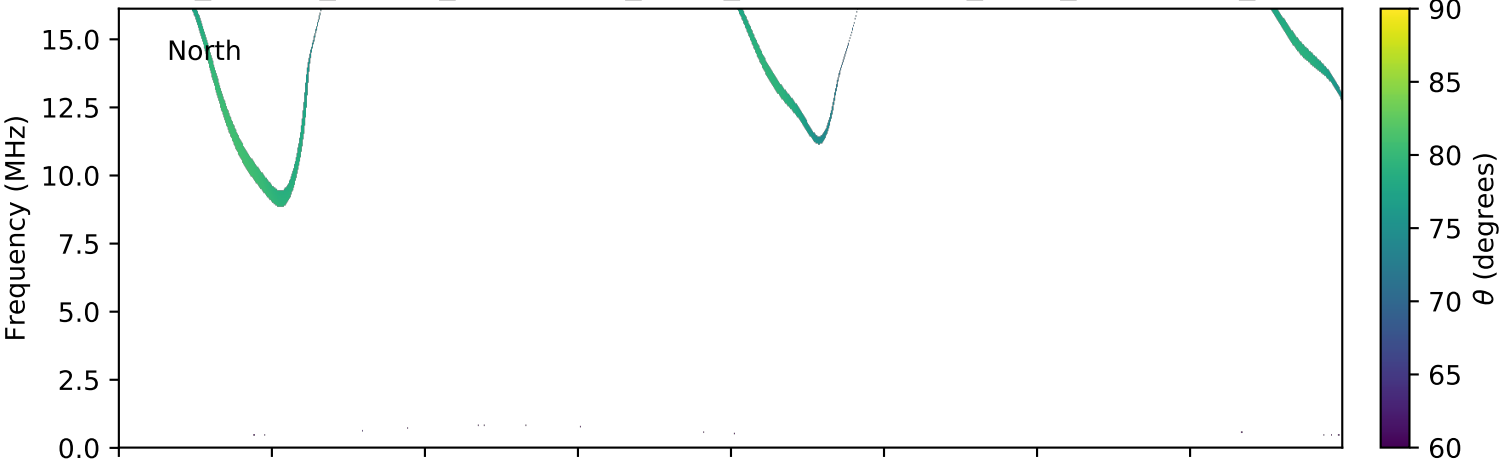
expres_cassini_jupiter_ganymede_isaac_lossc-wid1deg_3kev_20020820_v01.cdf
