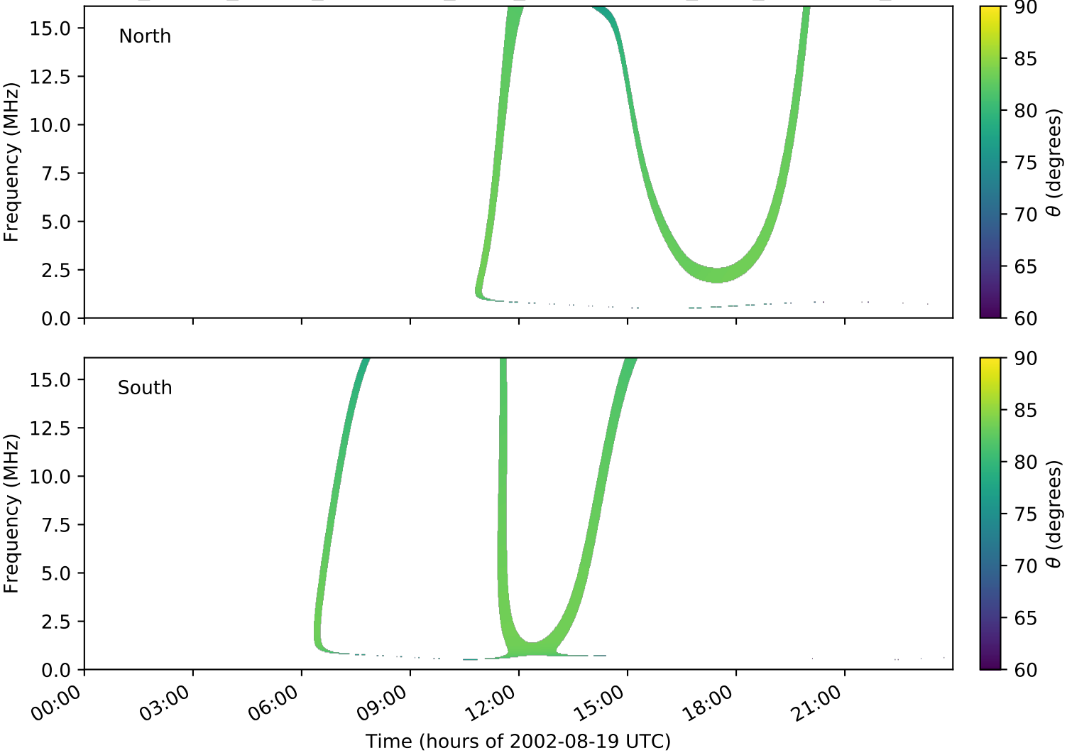
expres_cassini_jupiter_ganymede_isaac_lossc-wid1deg_3kev_20020819_v01.cdf
