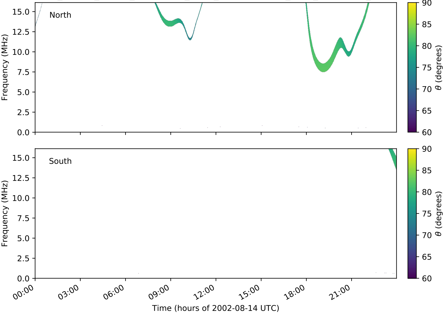
expres_cassini_jupiter_ganymede_isaac_lossc-wid1deg_3kev_20020814_v01.cdf
