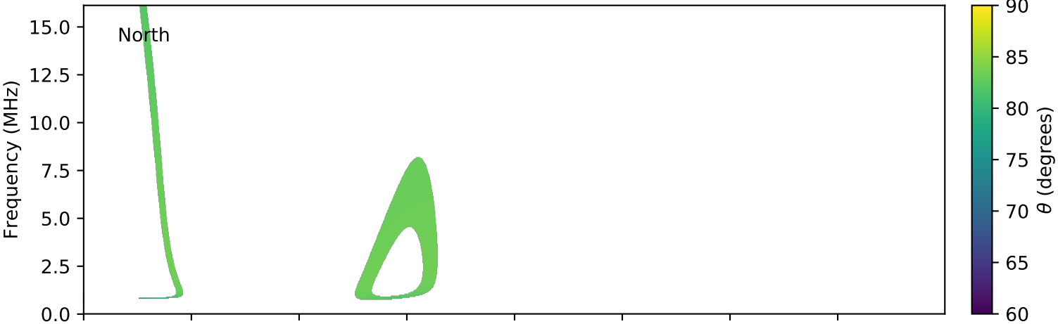
expres_cassini_jupiter_ganymede_isaac_lossc-wid1deg_3kev_20020808_v01.cdf
