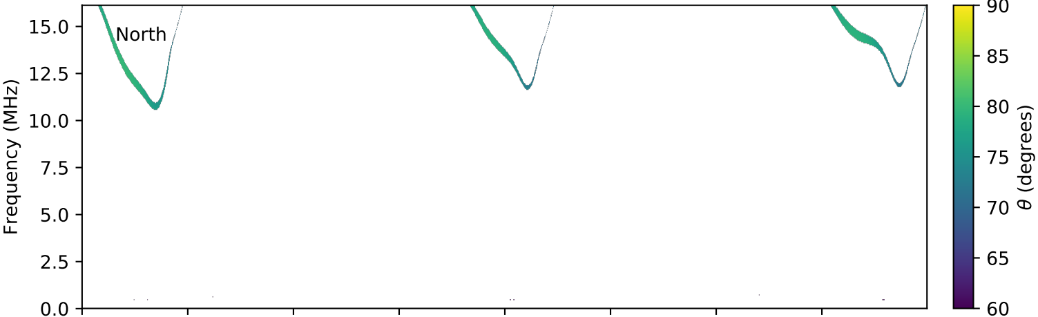
expres_cassini_jupiter_ganymede_isaac_lossc-wid1deg_3kev_20020806_v01.cdf
