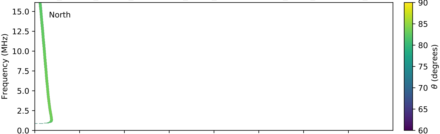
expres_cassini_jupiter_ganymede_isaac_lossc-wid1deg_3kev_20020801_v01.cdf
