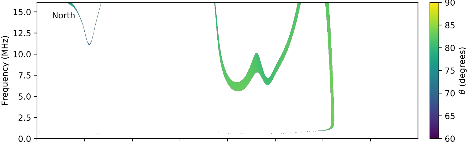
expres_cassini_jupiter_europa_isaac_lossc-wid1deg_3kev_20020830_v01.cdf
