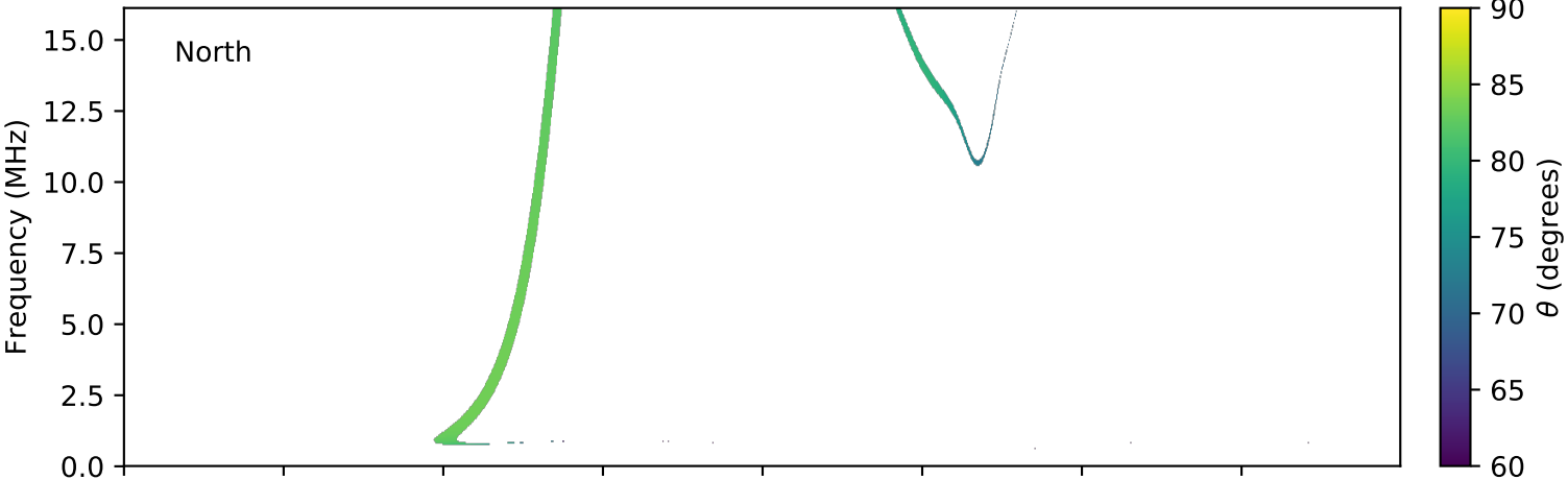
expres_cassini_jupiter_europa_isaac_lossc-wid1deg_3kev_20020829_v01.cdf
