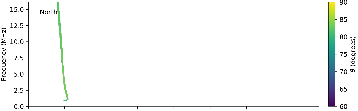
expres_cassini_jupiter_europa_isaac_lossc-wid1deg_3kev_20020827_v01.cdf
