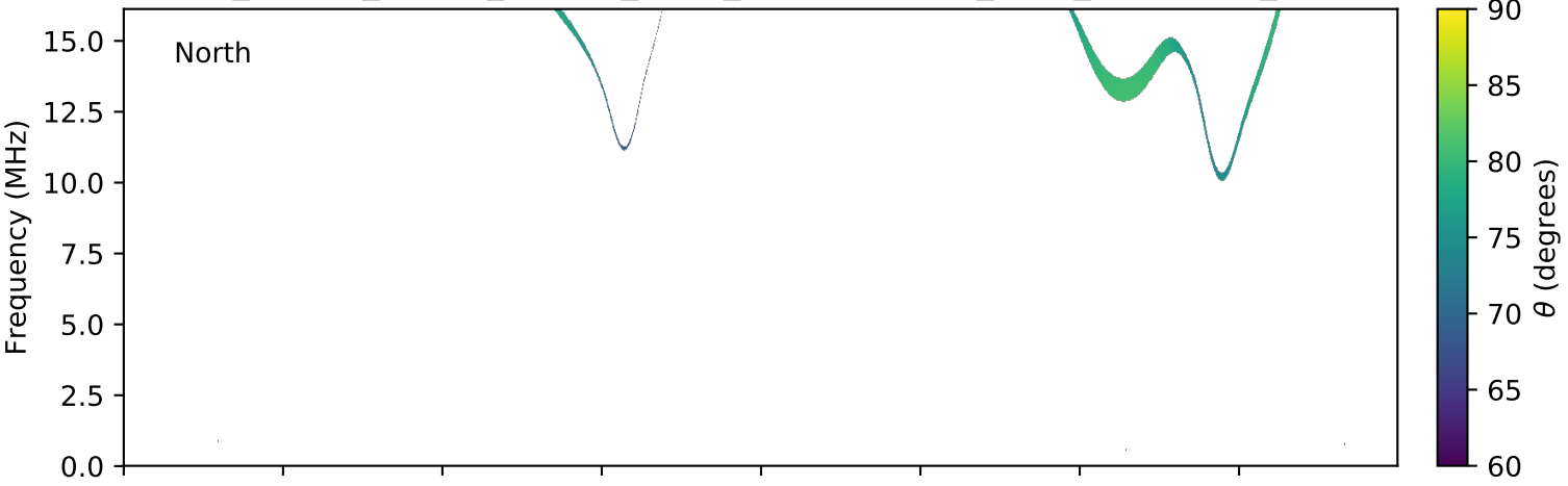
expres_cassini_jupiter_europa_isaac_lossc-wid1deg_3kev_20020826_v01.cdf
