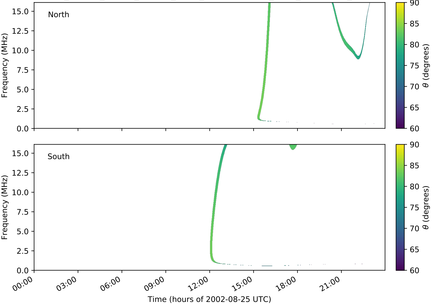
expres_cassini_jupiter_europa_isaac_lossc-wid1deg_3kev_20020825_v01.cdf
