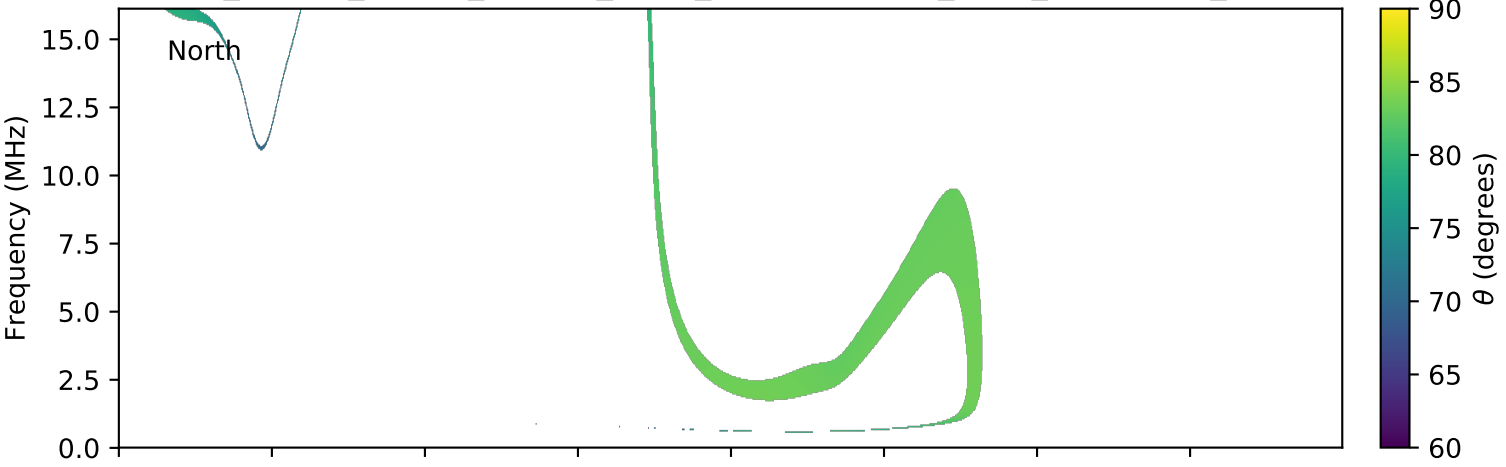
expres_cassini_jupiter_europa_isaac_lossc-wid1deg_3kev_20020823_v01.cdf
