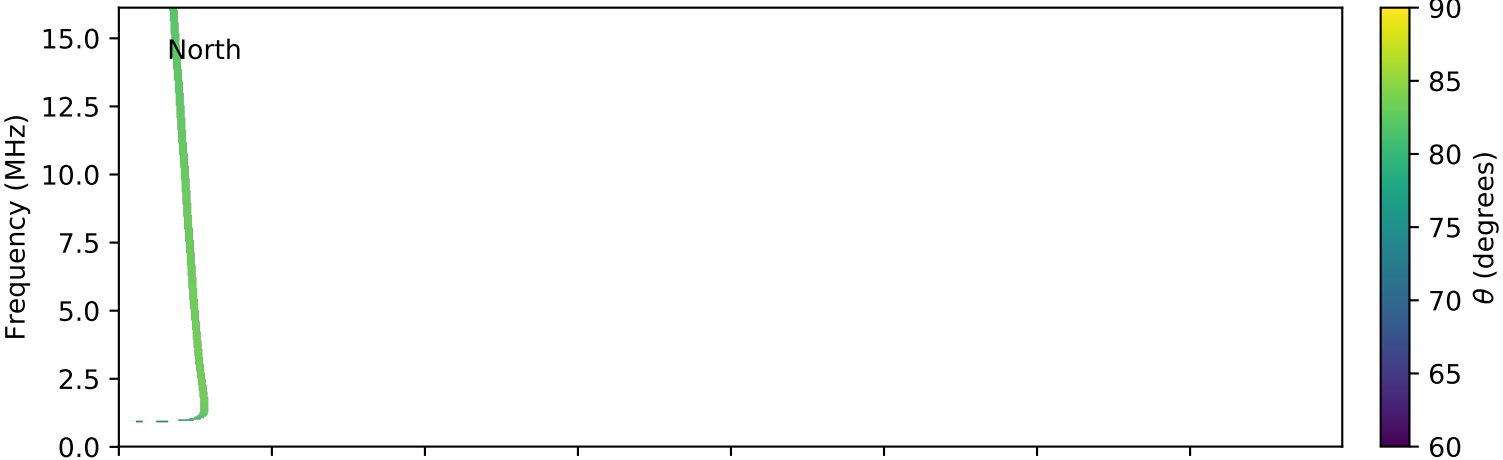
expres_cassini_jupiter_europa_isaac_lossc-wid1deg_3kev_20020820_v01.cdf
