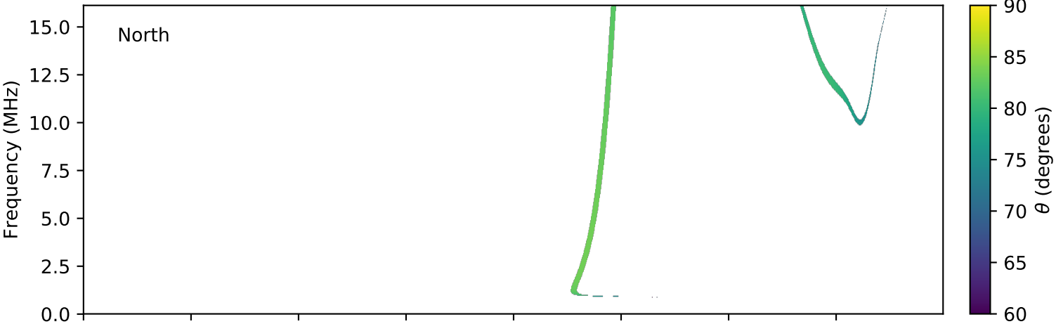
expres_cassini_jupiter_europa_isaac_lossc-wid1deg_3kev_20020818_v01.cdf
