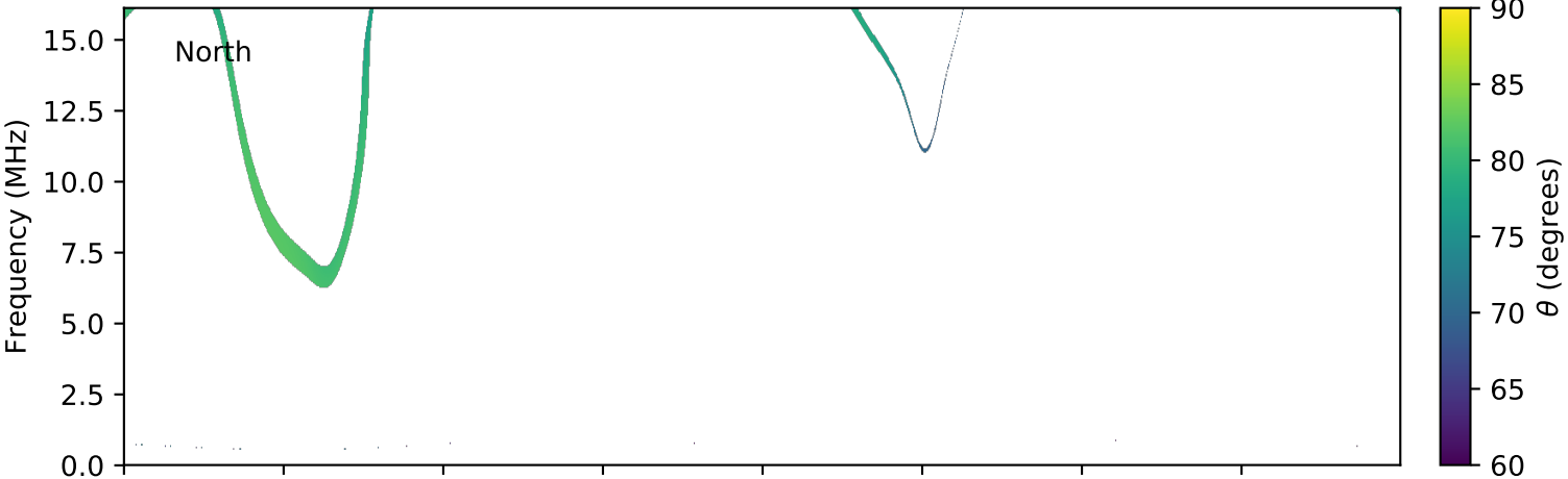
expres_cassini_jupiter_europa_isaac_lossc-wid1deg_3kev_20020815_v01.cdf
